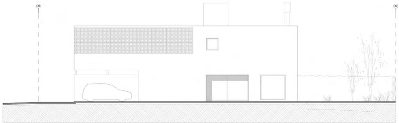
FACHADA LATERAL 0 1 2 3
